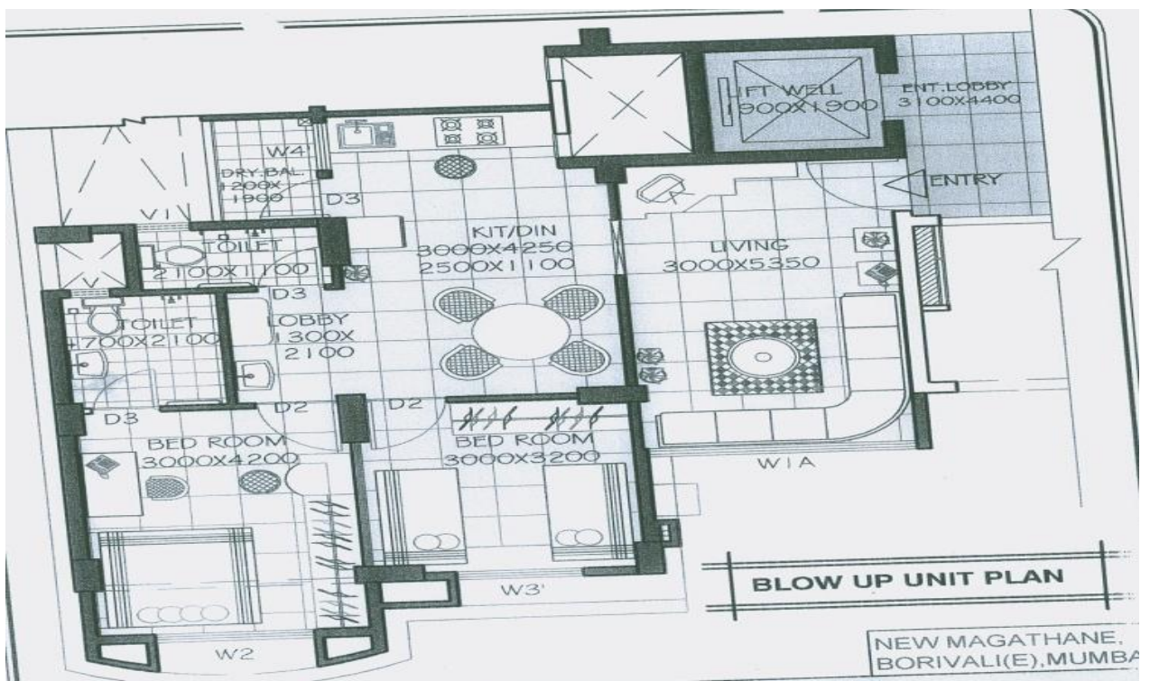
Typical Blown up unit Plan
