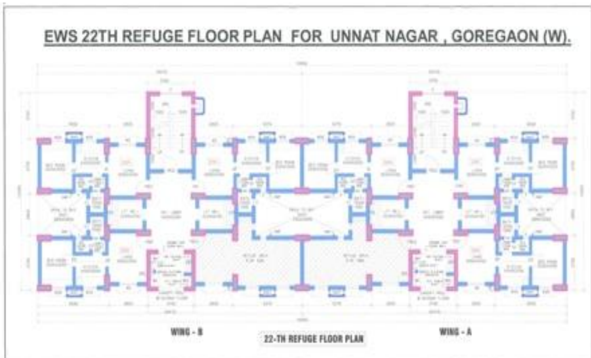
Typical Blown up unit Plan
